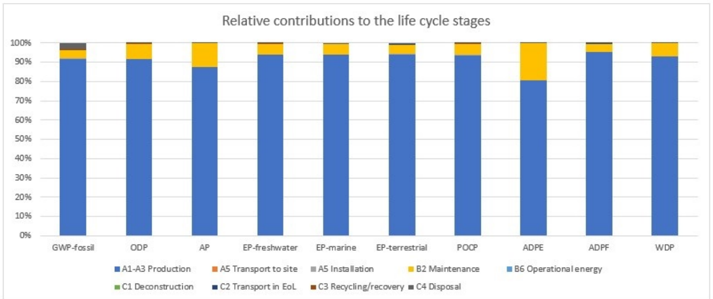
Figure 1: Relative environmental impacts of the different life cycle stages for the shutter SSL with solar-powered motor
