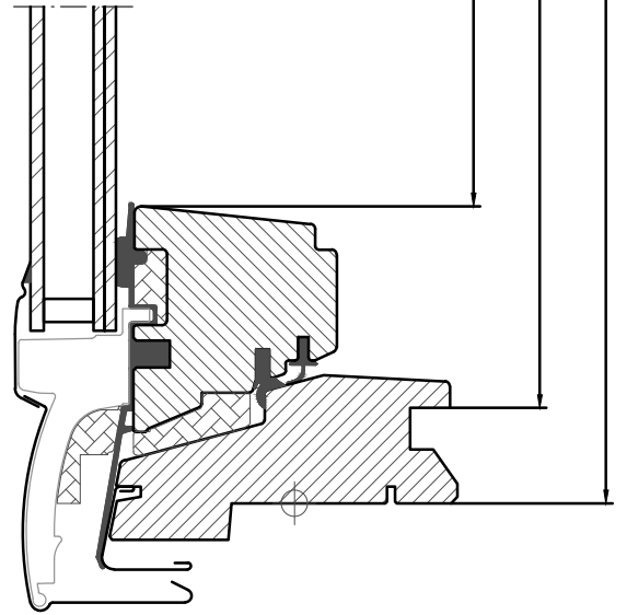
Fixed window
