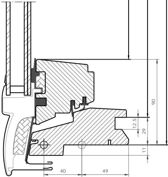
Pivot window
