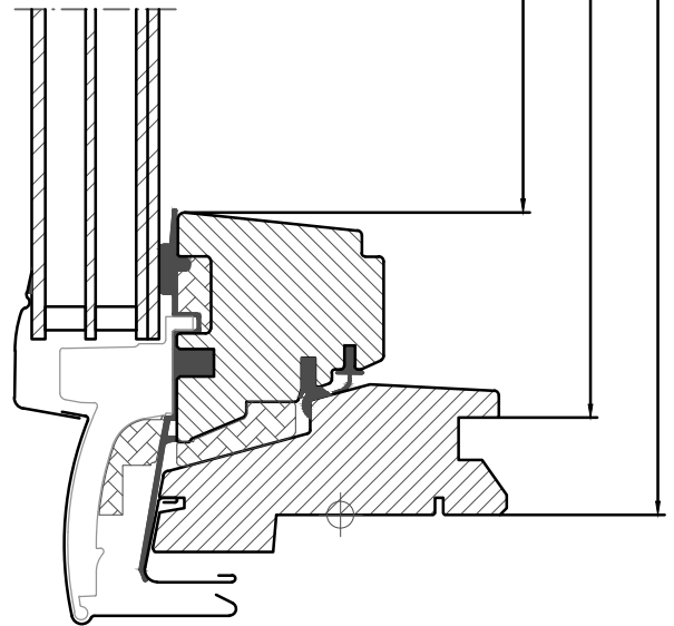
Fixed window
