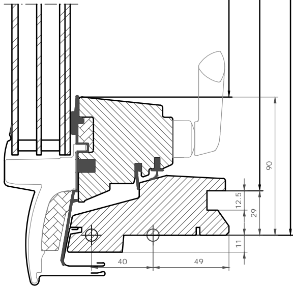
Top-hung window
