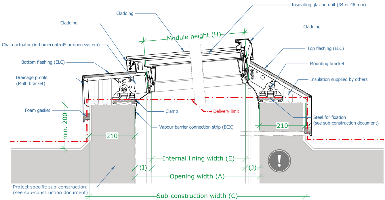
Cross-section - bottom
