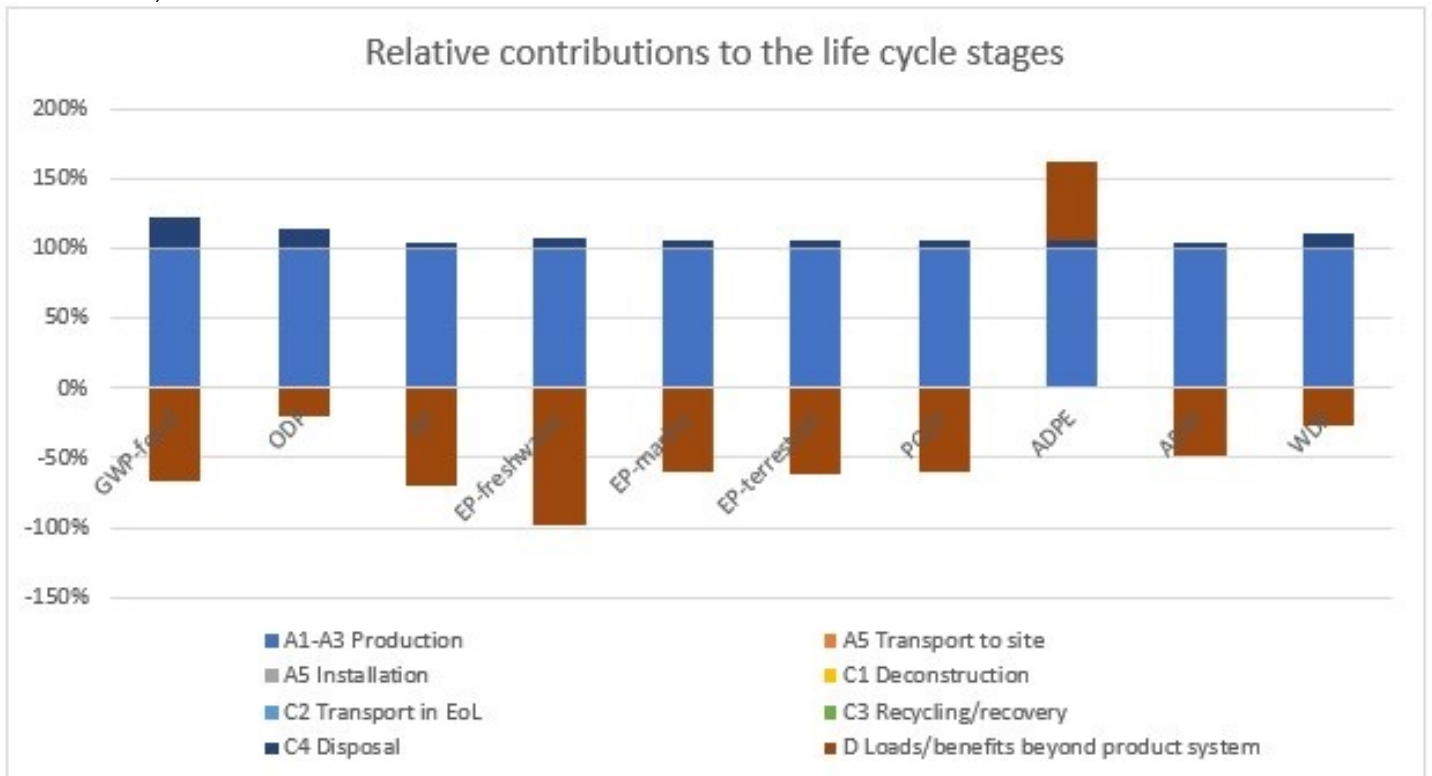
Figure 1: Relative environmental impacts of the different life cycle stages for the VELUX sun tunnel TCR 0K14 (Modules A1-A3 = 100%)
