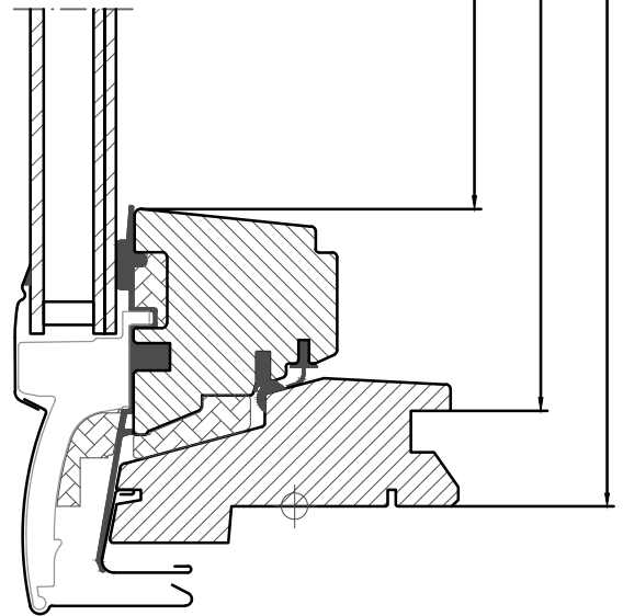
Fixed window
