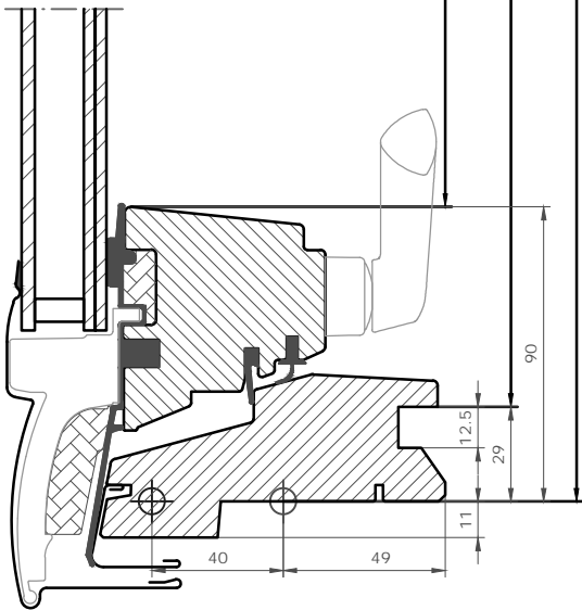
Top-hung window
