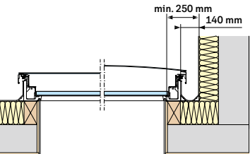
Minimum installation distances for fixed window (CFU)
