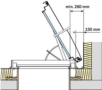
Minimum installation distances for electrically operated roof exit window (CXU)
